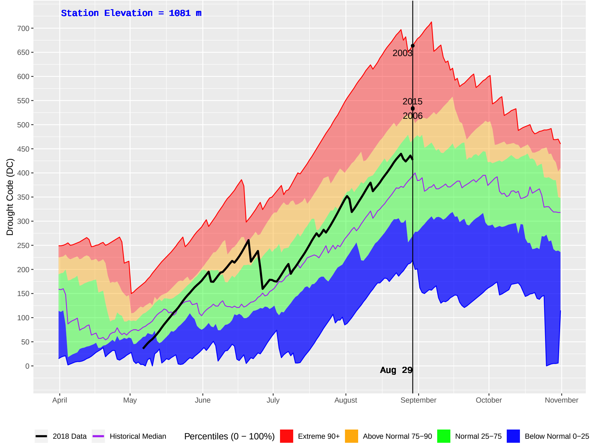
GAVIN (227) : Historical (1981–2016) and Current (2018) Daily Drought Code (DC)
