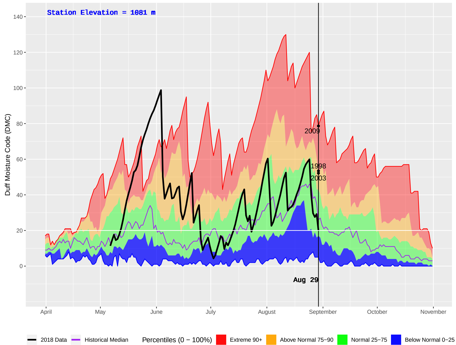
GAVIN (227) : Historical (1981–2016) and Current (2018) Daily Duff Moisture Code (DMC)
