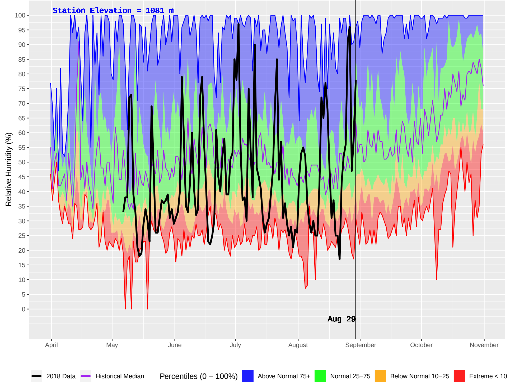
GAVIN (227) : Historical (1981–2016) and Current (2018) Daily Relative Humidity
