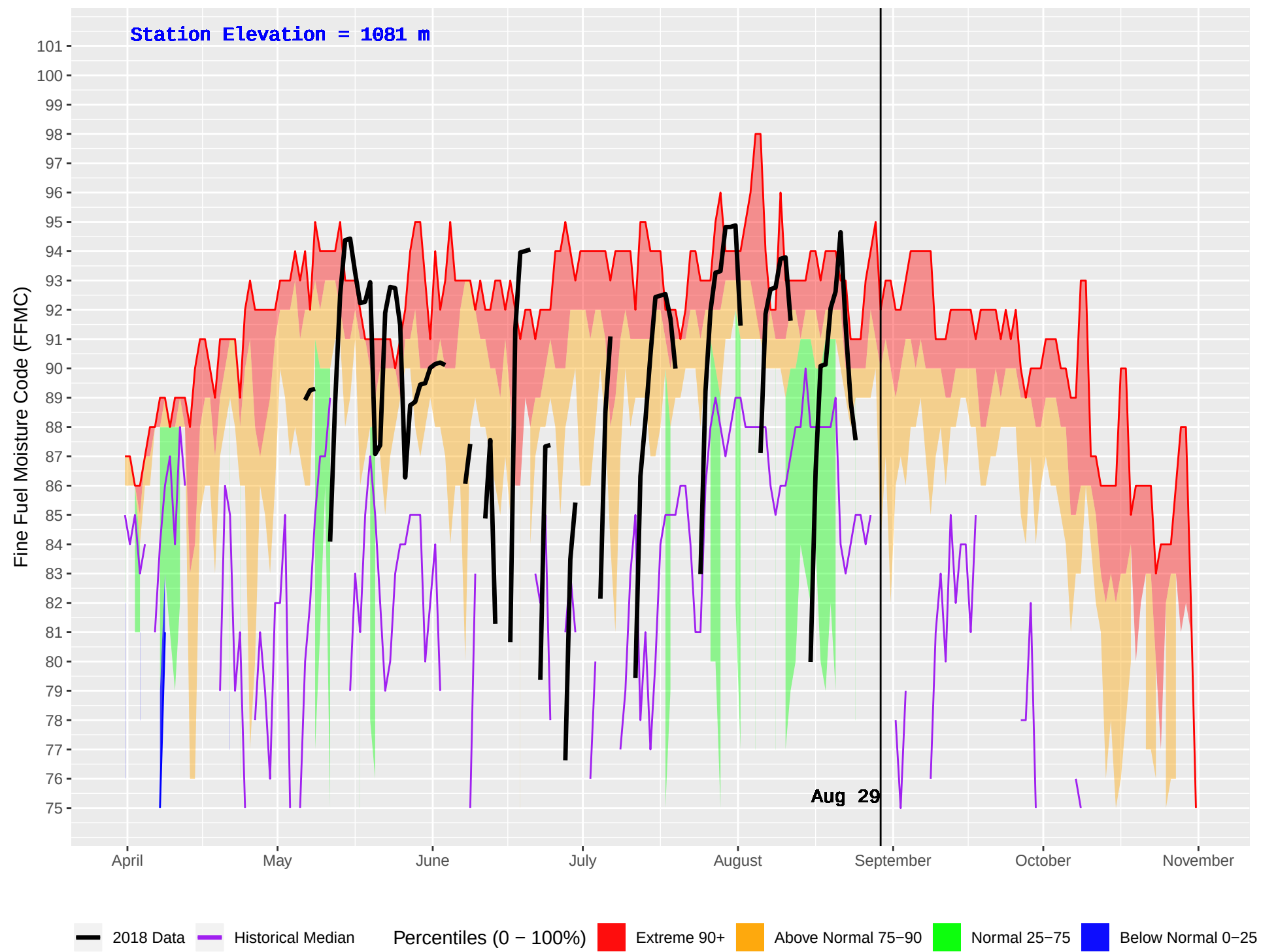
GAVIN (227) : Historical (1981–2016) and Current (2018) Daily Fine Fuel Moisture Code (FFMC)
