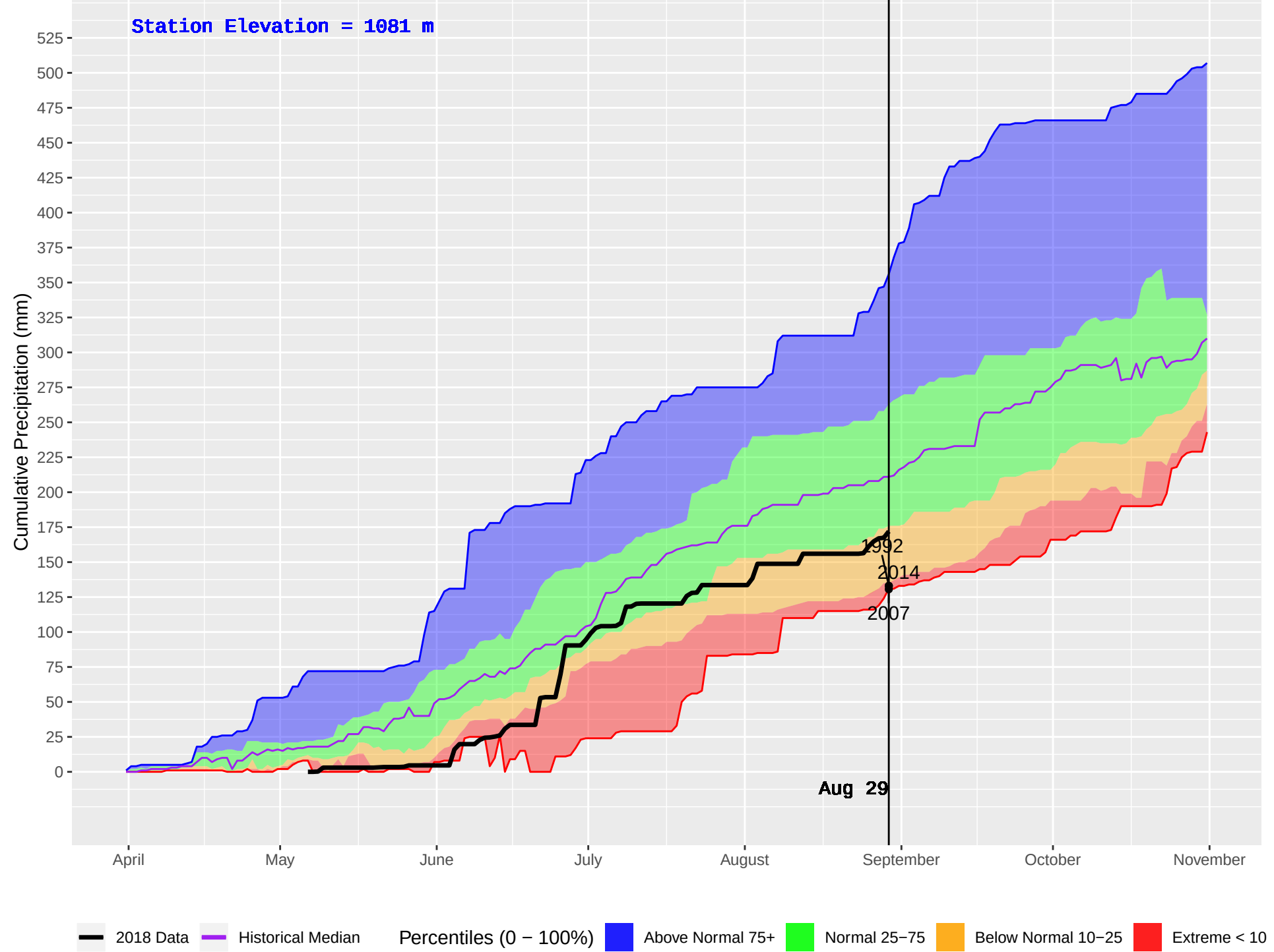
GAVIN (227) : Historical (1981–2016) and Current (2018) Daily Cumulative Precipitation
